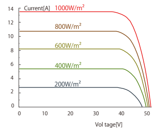
Current-Voltage Curve (550W)
