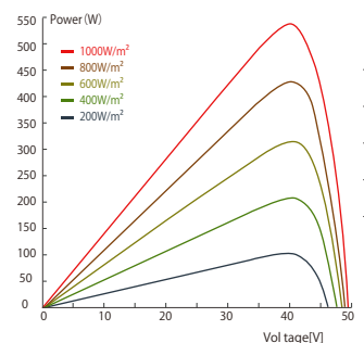
Power-Voltage Curve (550W)
